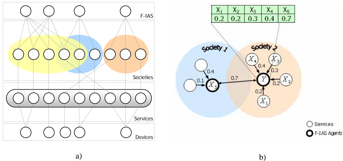
Figure 1. a) The Intelligent Association System Framework b) The structural concept of weighted fuzzy cognitive maps for F-IAS agents.
