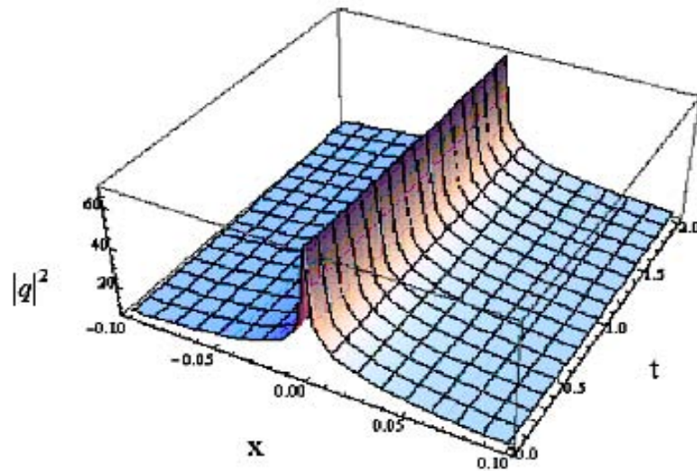
Figure 1: |q(x, t)|^2 for p = 3/2 and x is between -0.1 and 0.1 while t varies from 0.0 to 2.0 .
