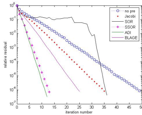
Fig.3 Comparison of convergent behavior of QMR method
