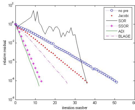
Fig.4 Comparison of convergent behavior of BiCG method
