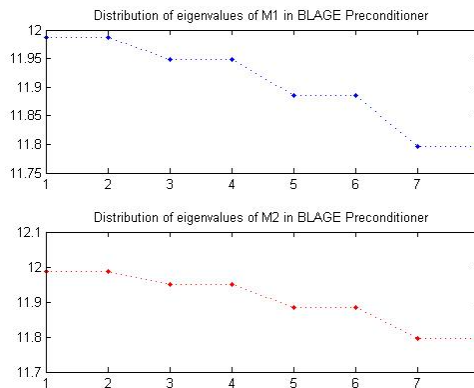
Fig.7 Distribution of eigenvalues in BLAGE Preconditioner
