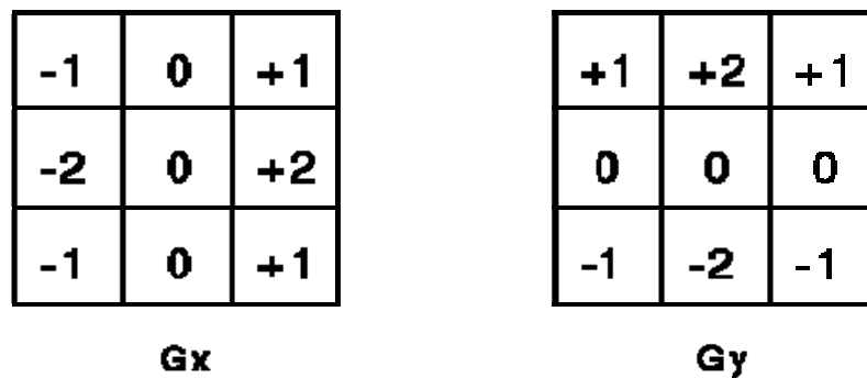
Fig. 1: Sobel operators
