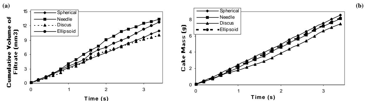
Fig. 3: (a) Cumulative volume of filtrate [mm 3 ] and (b) cake mass [g] vs. time [s]
