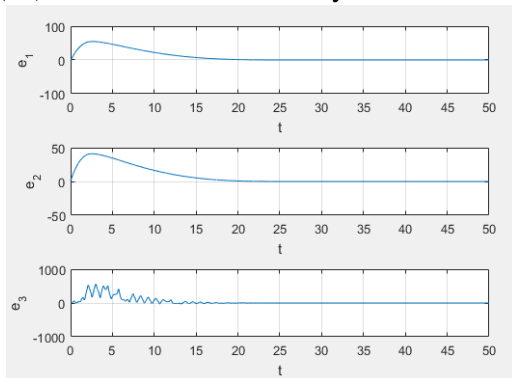
Fig.3 The error state time responses
