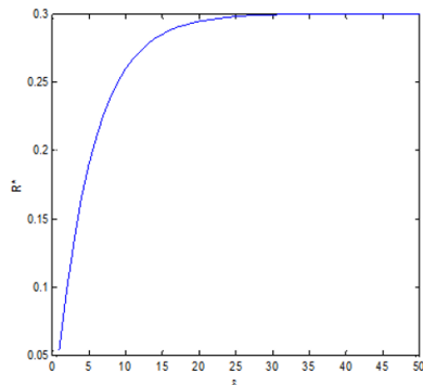
Figure 6a: \delta - R^* diagram
