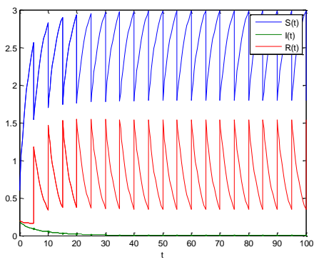
Figure 3: Emotions eventually stop spreading at p=0.4, R^* < 1
