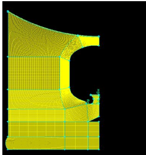
Fig.7 The grid model of the primary chamber
