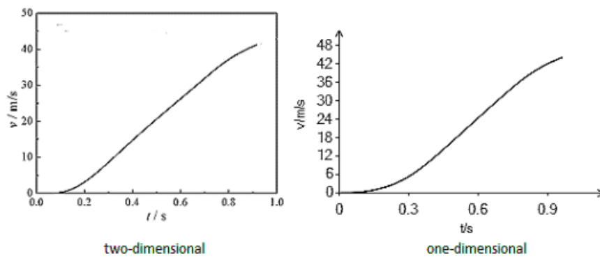
Fig.11 The velocity curve of the missile
