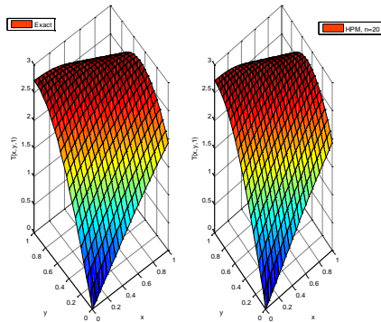
Fig. 4: The exact and numerical values of T(x, y, 1) .
