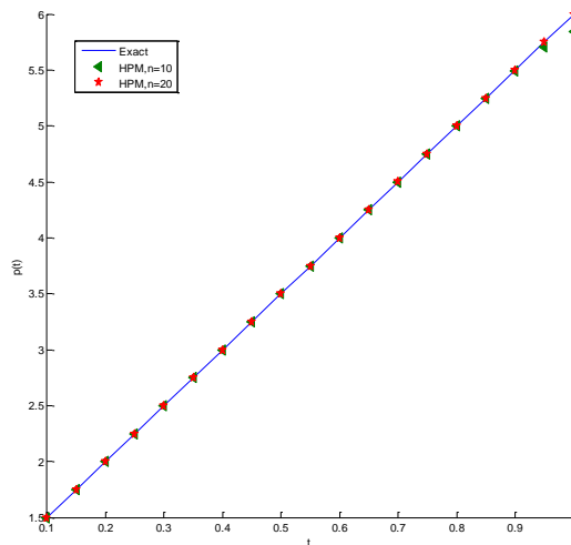
Fig. 5: The exact and numerical values of p(t) .
