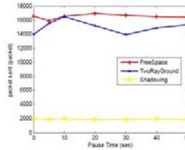
Fig. 9. Packet sent vs. pause time
