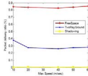
Fig. 7. Packet delivery ratio vs. speed
