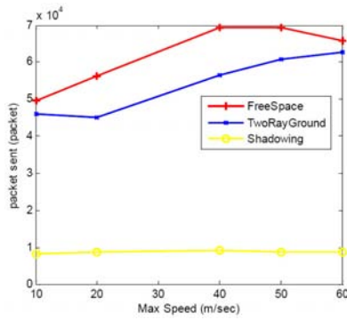
Fig. 4. Packet sent vs. speed
