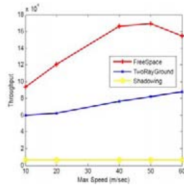
Fig. 5. Throughput vs. speed
