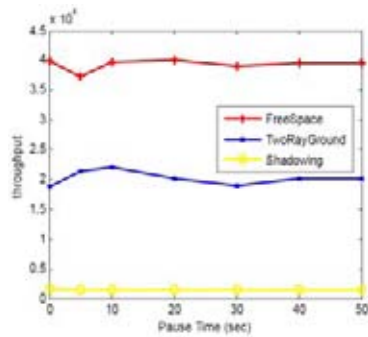
Fig. 10. Throughput vs. pause time
