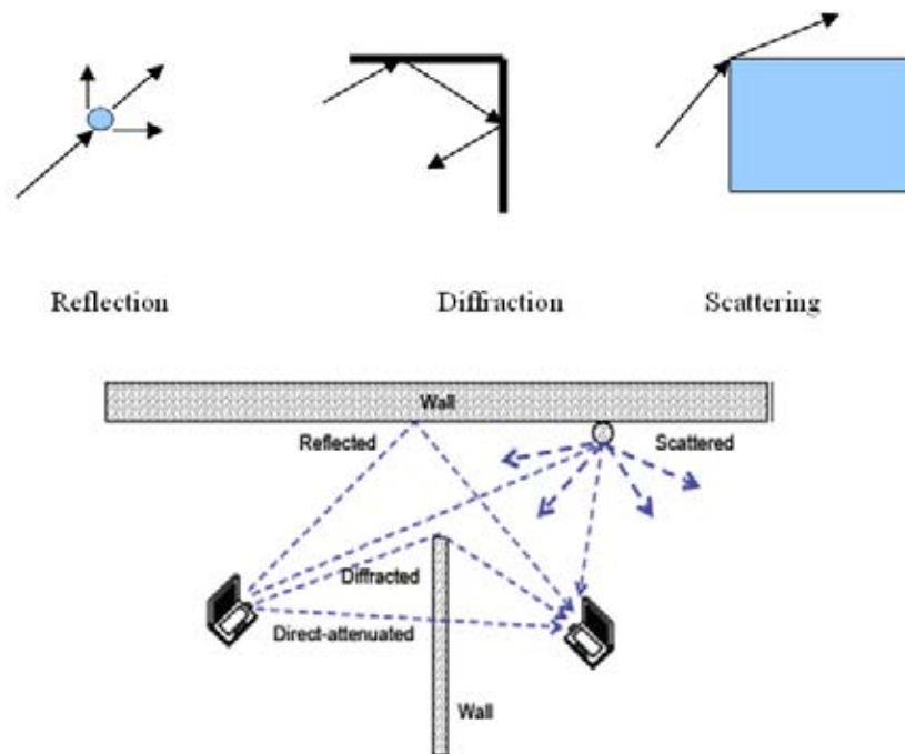
Fig. 1. The phenomena effect radio wave propagation
