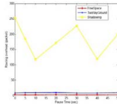
Fig. 13. Routing overhead vs. pause time
