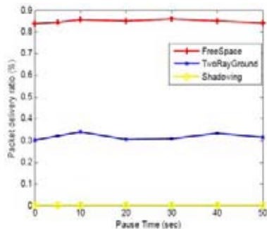
Fig. 12. Packet delivery ratio vs. pause time
